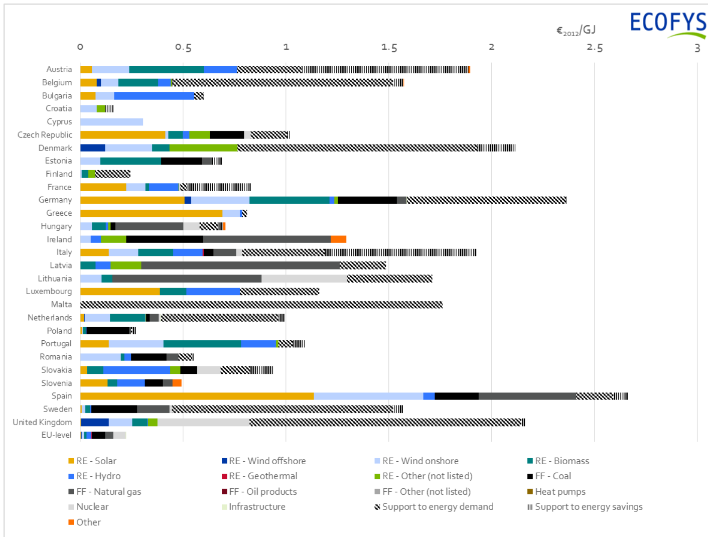
Figure S - 4 Interventions by Member State per unit of primary energy demand (GJ) in 2012 3 Note: The EU-level intervention refers to interventions financed by the EU and not by individual Member States.
